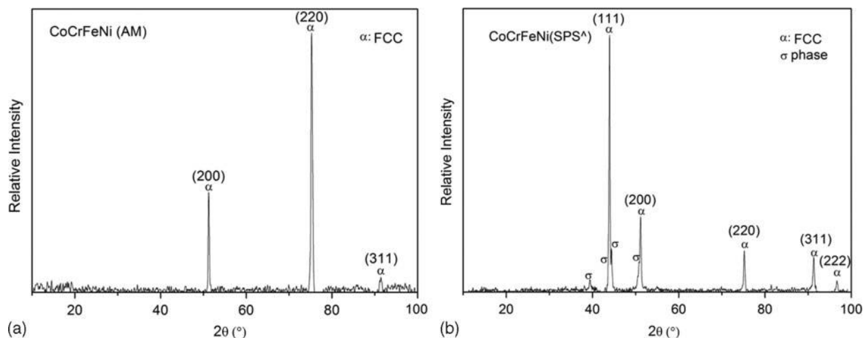
5 XRD pattern for a as cast CoCrFeNi (AM) and b as cast CoCrFeNi (SPS A )
